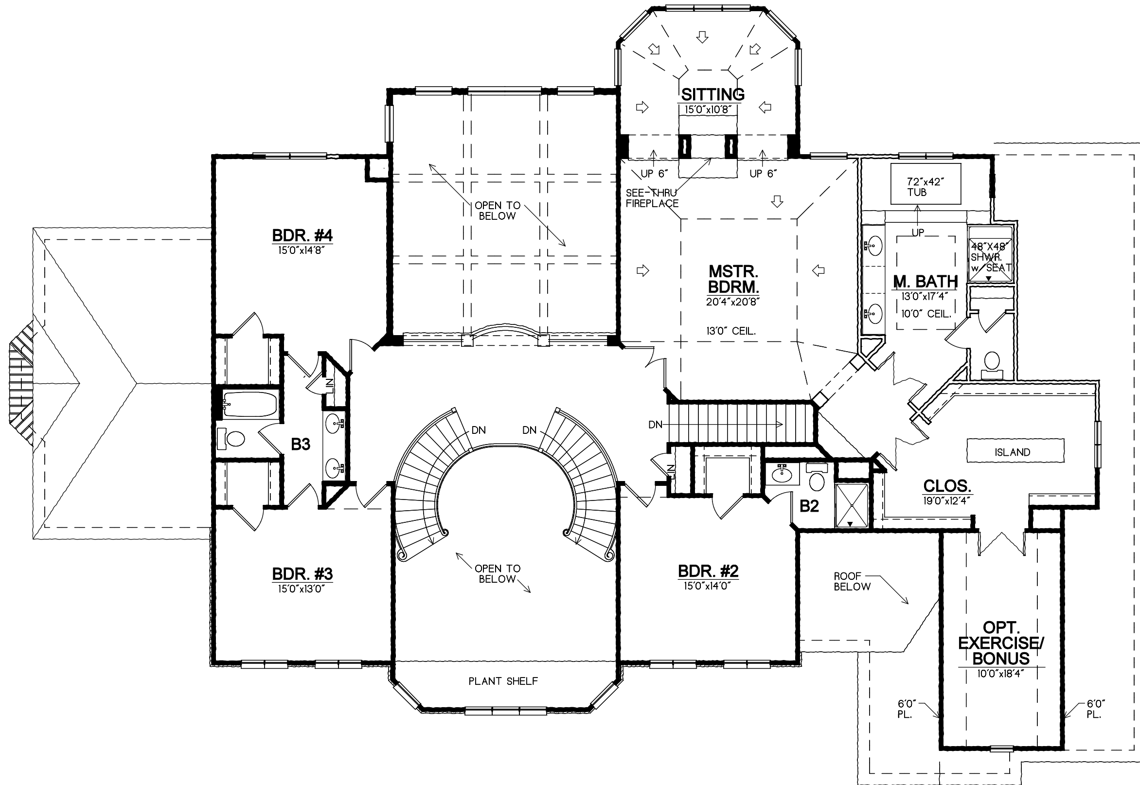
2nd Floor Scale: 1/8"=1'-0"
